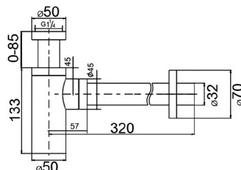
BS197-B - Bottle 'P' Trap - Matt Black
