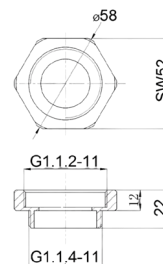
BS197AD - Adapter 40-32mm suit Bottle 'P' Trap - Chrome
