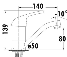
PM-1001SWC - Ruby Swivel Basin Mixer - Chrome
