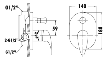
PM-3002SW - Ruby Wall Mixer w\ Diverter - Chrome
