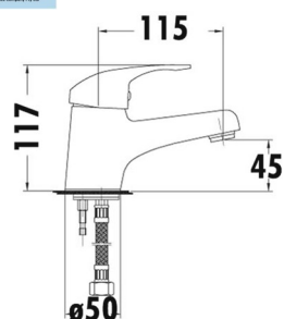
PM-2001SW - Ruby Basin Mixer - Chrome
