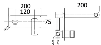
PSL3003 - Eden Wall Mixer with Outlet - Chrome
