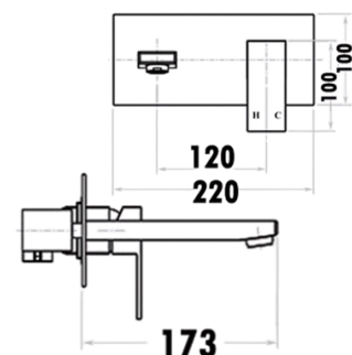
PSS3003SB - Nova Wall Mixer with Outlet - Chrome
