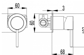
HYB88-301-60 - Hali Wall Mixer 60mm Back Plate - Chrome
