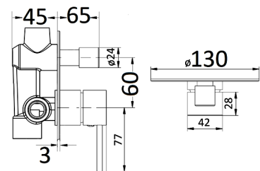
HYB88-501 - Hali Wall Mixer with Diverter - Chrome
