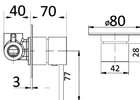
HYB88-301 - Hali Wall Mixer - Chrome
