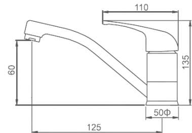
DMB2- Demos Swivel Basin Mixer - Chrome
