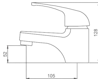
DMB1 - Demos Basin Mixer - Chrome
